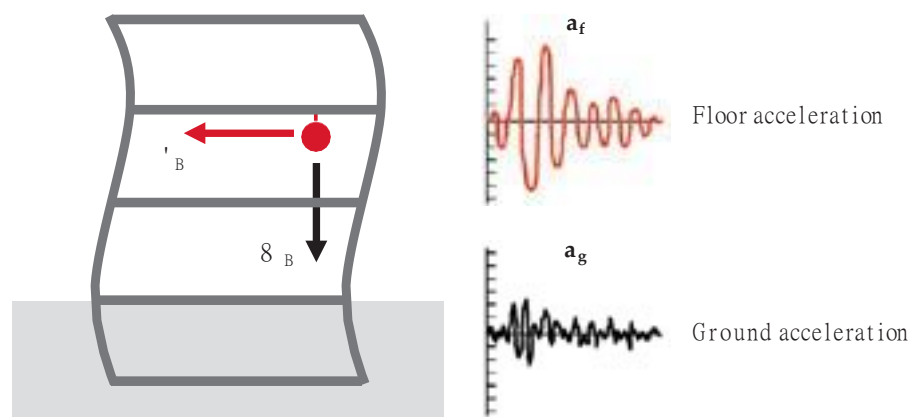
Fig. 2.1 Equivalent static analysis for the determination of earthquake actions on non-structural elements
