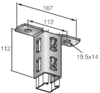
Connector MQV-2/2D-14 Itemn.: 369639
